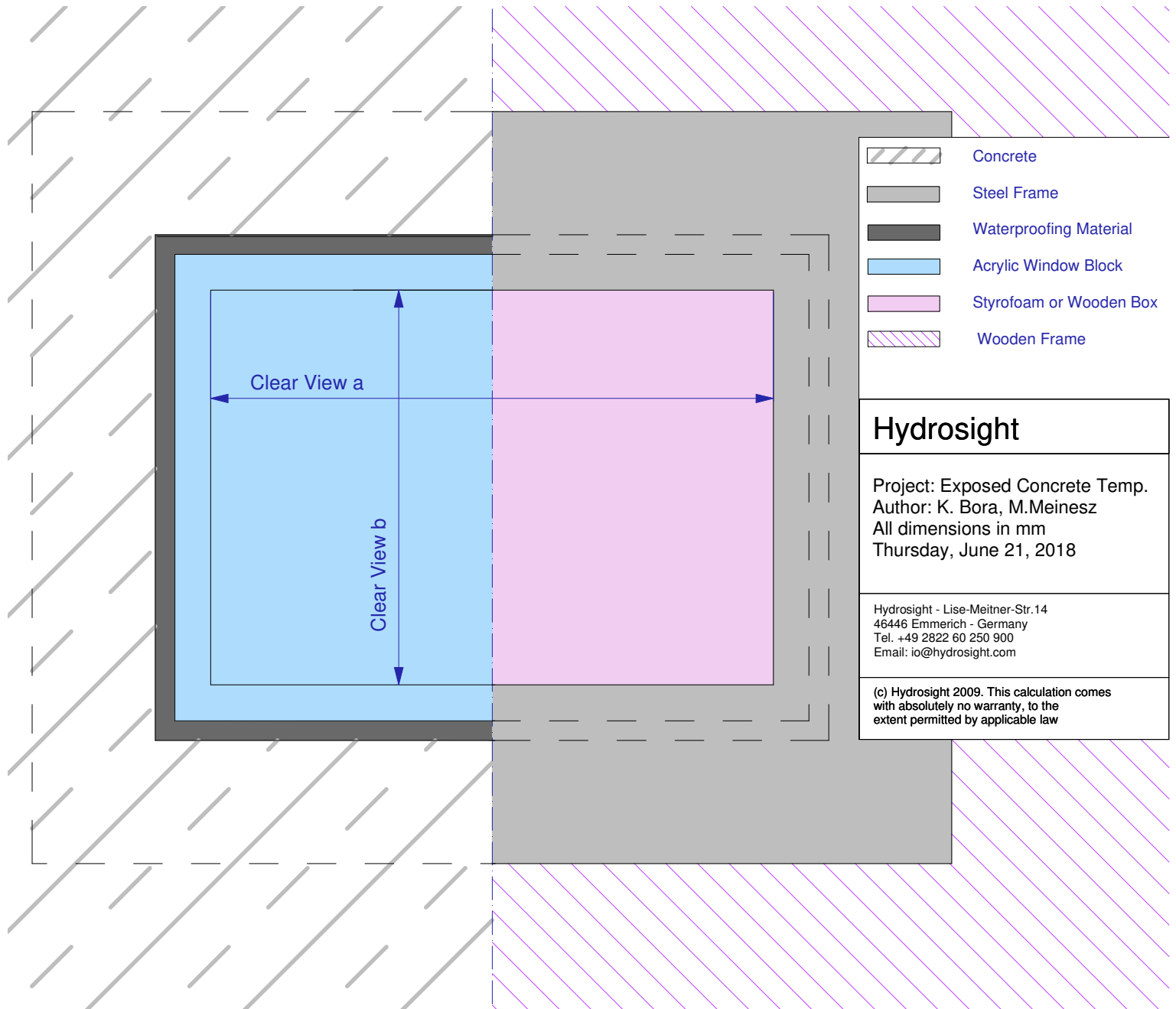
Cross Section when finished
